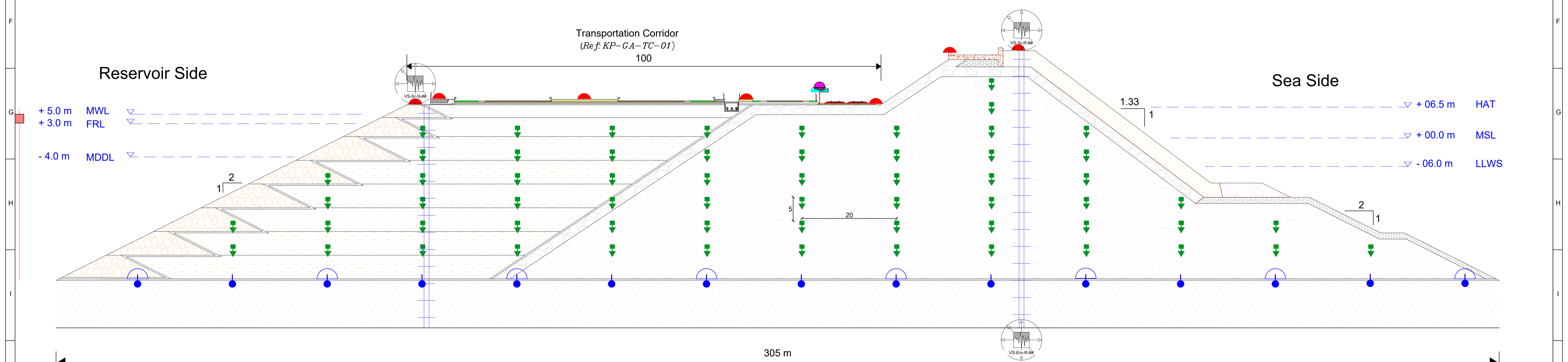
CROSS SECTION OF KALAPASAR DAM
